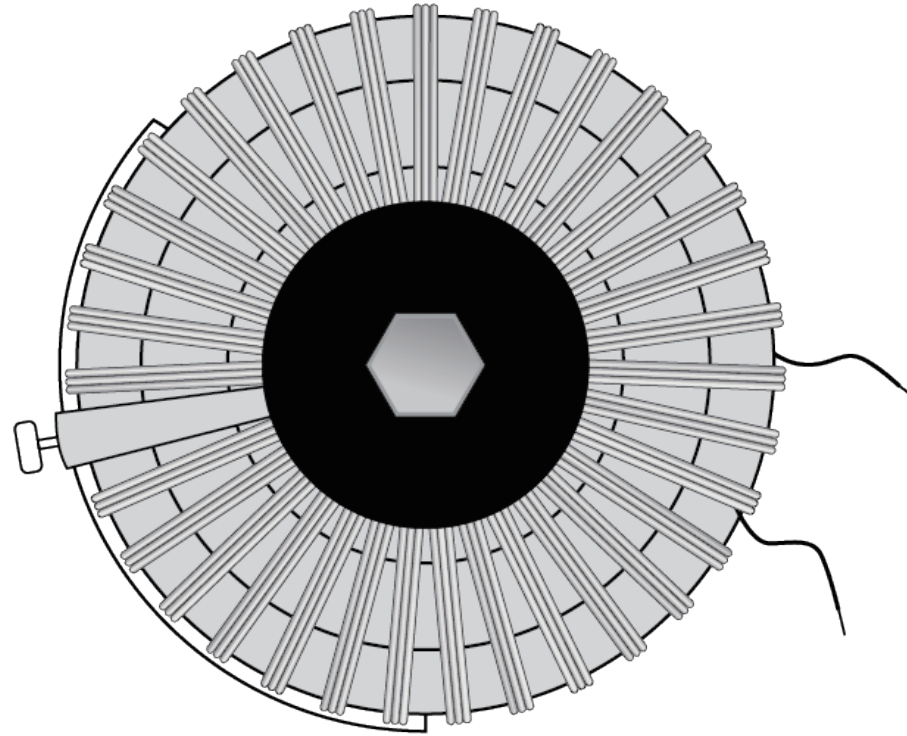
Toroidal transformer
